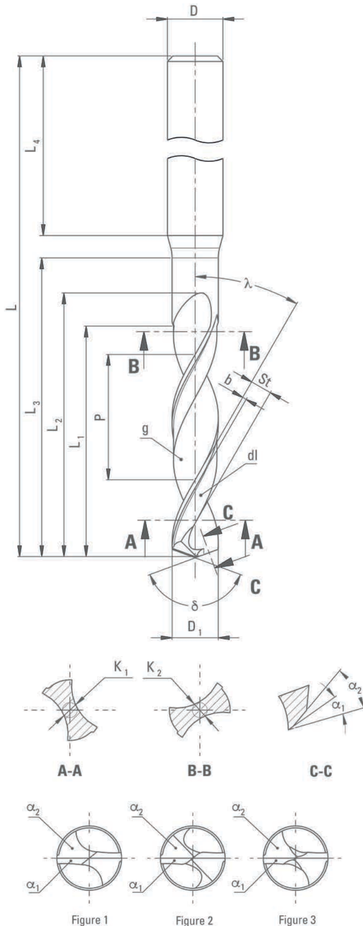
Figure 1 : Drill with web thinning
